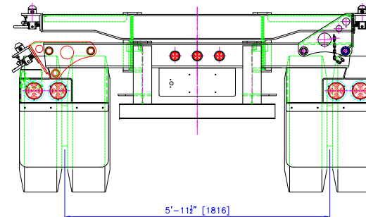
VIEW A 1:25
