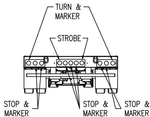
REAR VIEW
